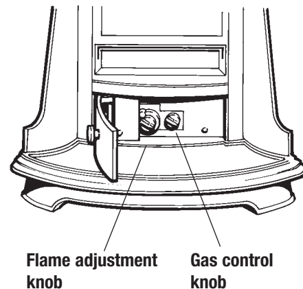
Illustration 15.2 To ignite the pilot, use the two controls indicated above.
