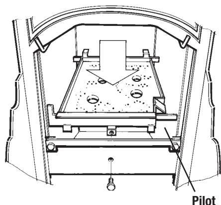
Illustration 15.5 When the pilot is lit, the flame will be clearly visible at the right side of the firebox, beneath the right side of the burner pan.
